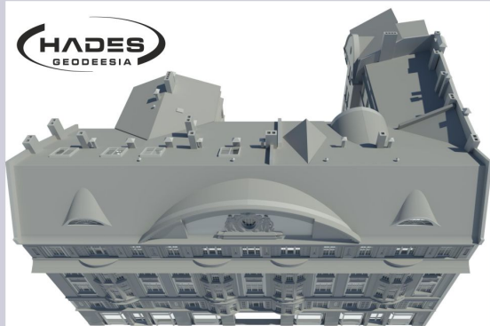
Facade 3D CAD Model from Point Cloud
